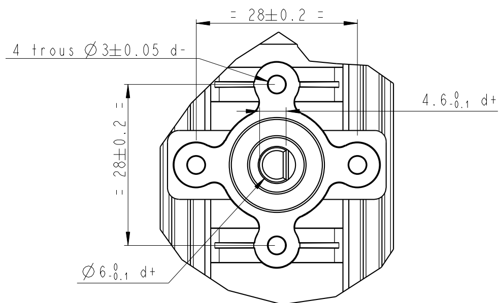
DETAIL A ECHELLE 3/2
